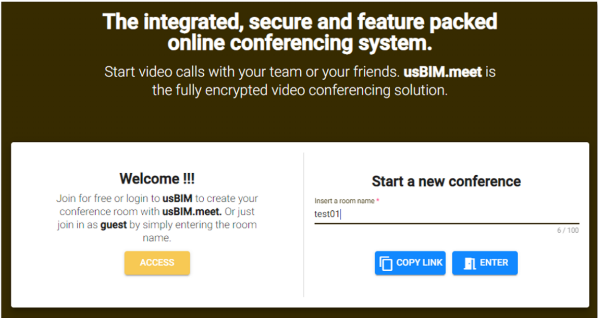
Figure 2. Room Creation
