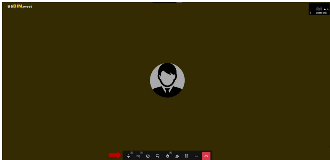
Figure 4. Meeting Screen
