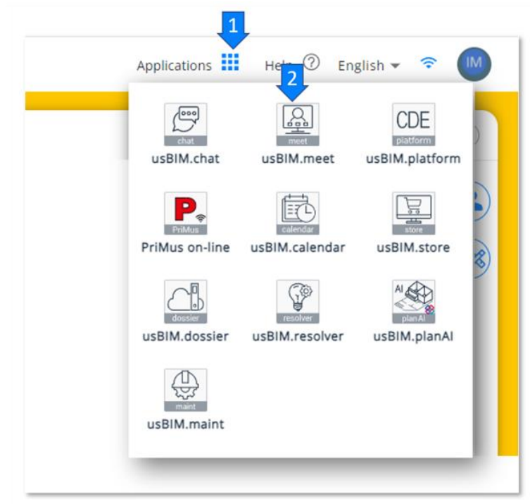
Figure 1. UsBIM.meet section
