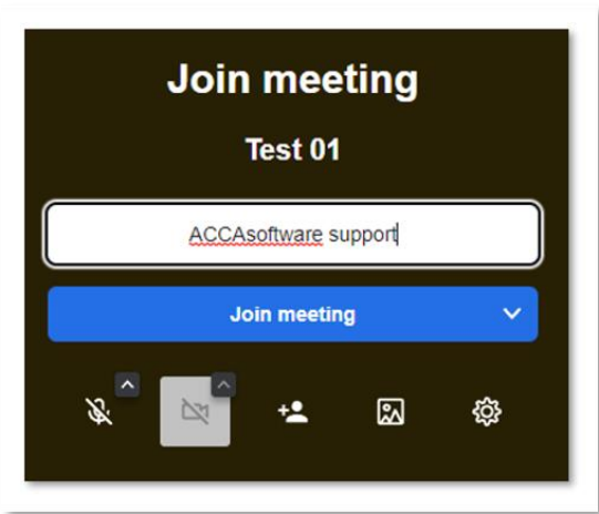
Figure 3. Start Meeting
